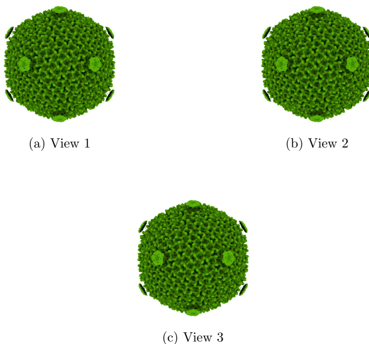
Figure 4: Isosurface at threshold=5760.000000. Views generated by ChimeraX at the following X, Y, Z angles: View 1 (0, -90, -90), View 2 (-90, 0, -90), View 3 (0, 0, 0).
