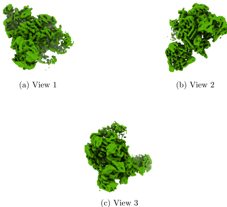
Figure 4: Isosurface at threshold=0.008140. Views generated by ChimeraX at a the following X, Y, Z angles: View 1 (0, -90, -90), View 2 (-90, 0, -90), View 3 (0, 0, 0).
