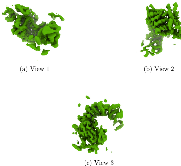
Figure 4: Isosurface at threshold=0.044900. Views generated by ChimeraX at a the following X, Y, Z angles: View 1 (0, -90, -90), View 2 (-90, 0, -90), View 3 (0, 0, 0).
