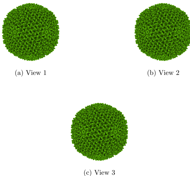
Figure 4: Isosurface at threshold=5260.000000. Views generated by ChimeraX at the following X, Y, Z angles: View 1 (0, -90, -90), View 2 (-90, 0, -90), View 3 (0, 0, 0).
