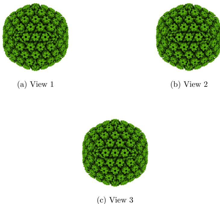
Figure 4: Isosurface at threshold=83.500000. Views generated by ChimeraX at a the following X, Y, Z angles: View 1 (0, -90, -90), View 2 (-90, 0, -90), View 3 (0, 0, 0).
