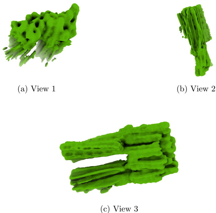
Figure 4: Isosurface at threshold=0.025800. Views generated by ChimeraX at a the following X, Y, Z angles: View 1 (0, -90, -90), View 2 (-90, 0, -90), View 3 (0, 0, 0).
