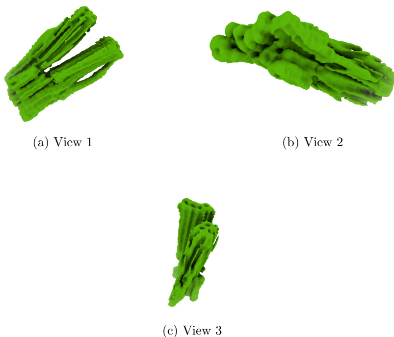
Figure 4: Isosurface at threshold=0.020600. Views generated by ChimeraX at a the following X, Y, Z angles: View 1 (0, -90, -90), View 2 (-90, 0, -90), View 3 (0, 0, 0).
