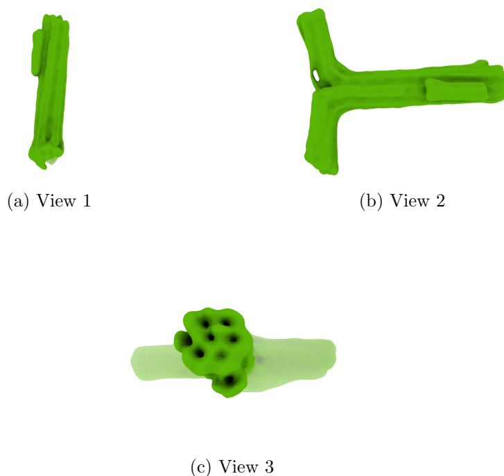
Figure 4: Isosurface at threshold=0.054400. Views generated by ChimeraX at a the following X, Y, Z angles: View 1 (0, -90, -90), View 2 (-90, 0, -90), View 3 (0, 0, 0).
