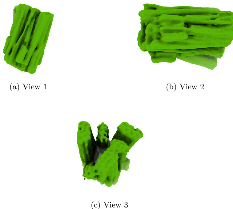
Figure 4: Isosurface at threshold=0.027900. Views generated by ChimeraX at a the following X, Y, Z angles: View 1 (0, -90, -90), View 2 (-90, 0, -90), View 3 (0, 0, 0).
