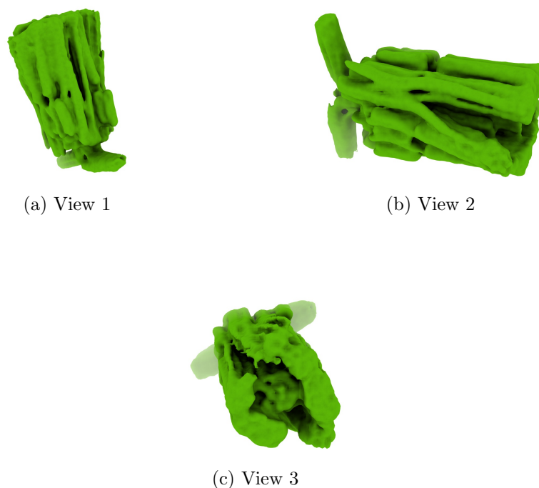
Figure 4: Isosurface at threshold=0.032600. Views generated by ChimeraX at a the following X, Y, Z angles: View 1 (0, -90, -90), View 2 (-90, 0, -90), View 3 (0, 0, 0).
