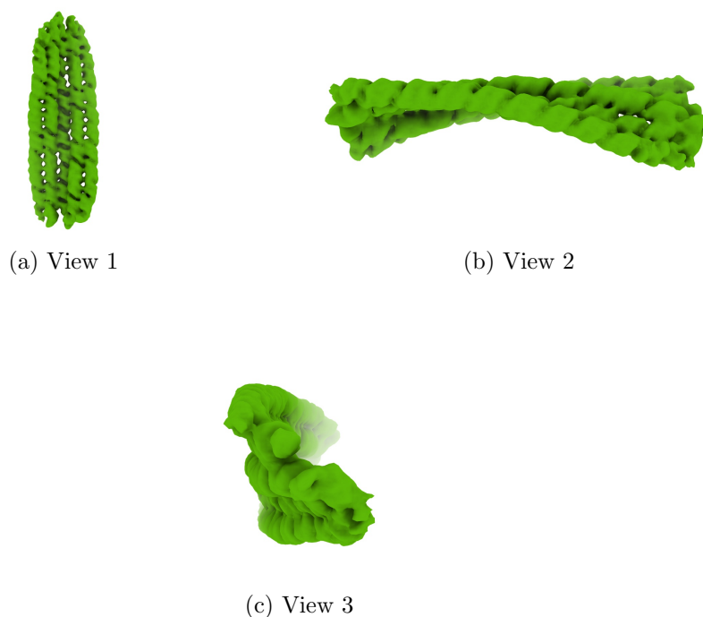
Figure 4: Isosurface at threshold=2.250000. Views generated by ChimeraX at a the following X, Y, Z angles: View 1 (0, -90, -90), View 2 (-90, 0, -90), View 3 (0, 0, 0).
