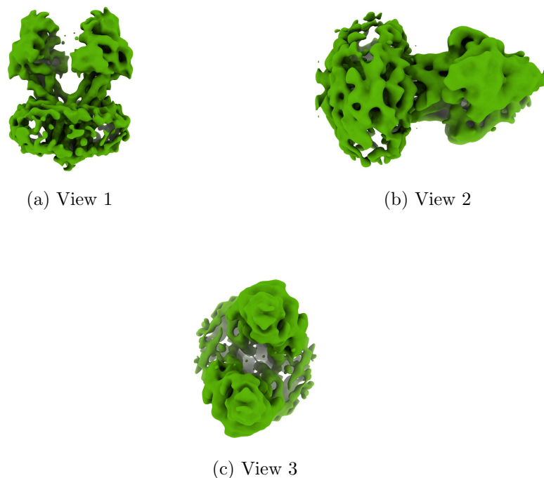
Figure 4: Isosurface at threshold=0.170400. Views generated by ChimeraX at a the following X, Y, Z angles: View 1 (0, -90, -90), View 2 (-90, 0, -90), View 3 (0, 0, 0).
