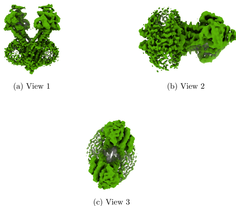
Figure 4: Isosurface at threshold=0.186800. Views generated by ChimeraX at a the following X, Y, Z angles: View 1 (0, -90, -90), View 2 (-90, 0, -90), View 3 (0, 0, 0).
