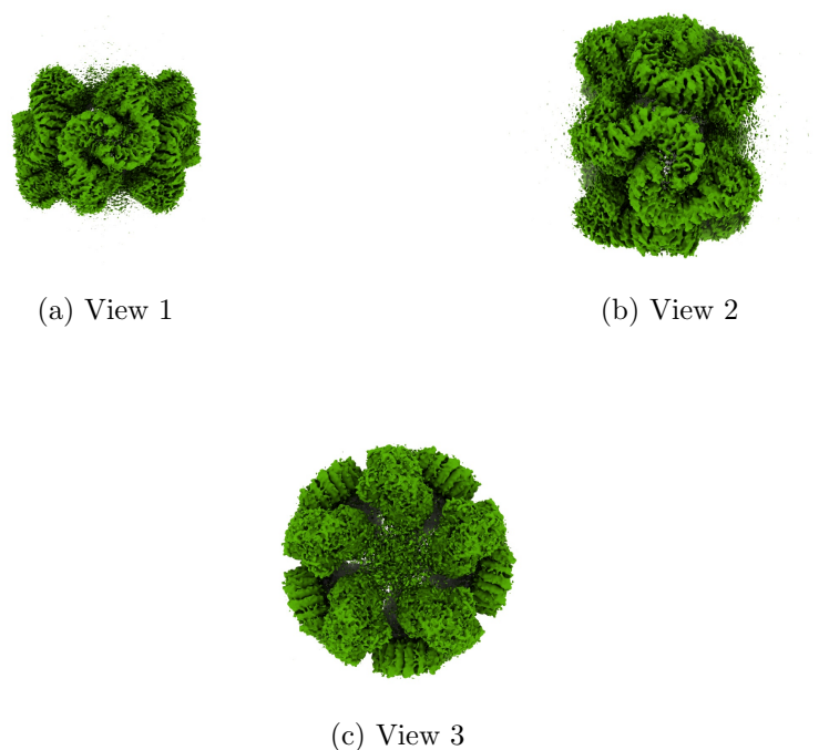
Figure 4: Isosurface at threshold=0.005150. Views generated by ChimeraX at the following X, Y, Z angles: View 1 (0, -90, -90), View 2 (-90, 0, -90), View 3 (0, 0, 0).
