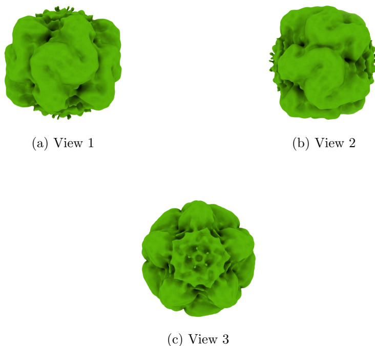
Figure 4: Isosurface at threshold=0.002860. Views generated by ChimeraX at a the following X, Y, Z angles: View 1 (0, -90, -90), View 2 (-90, 0, -90), View 3 (0, 0, 0).
