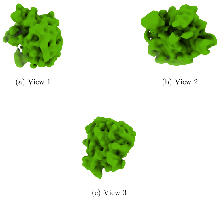
Figure 4: Isosurface at threshold=0.000394. Views generated by ChimeraX at a the following X, Y, Z angles: View 1 (0, -90, -90), View 2 (-90, 0, -90), View 3 (0, 0, 0).
