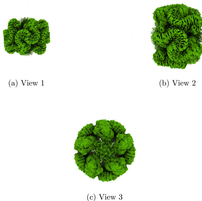
Figure 4: Isosurface at threshold=0.068000. Views generated by ChimeraX at a the following X, Y, Z angles: View 1 (0, -90, -90), View 2 (-90, 0, -90), View 3 (0, 0, 0).
