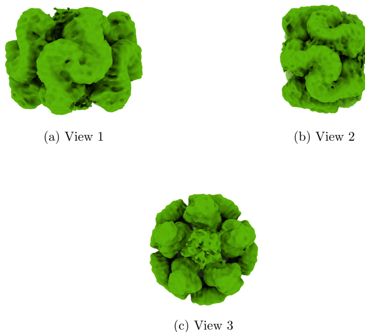
Figure 4: Isosurface at threshold=0.041700. Views generated by ChimeraX at a the following X, Y, Z angles: View 1 (0, -90, -90), View 2 (-90, 0, -90), View 3 (0, 0, 0).
