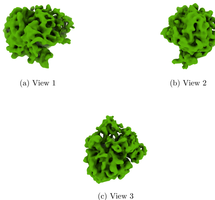
Figure 4: Isosurface at threshold=0.000369. Views generated by ChimeraX at a the following X, Y, Z angles: View 1 (0, -90, -90), View 2 (-90, 0, -90), View 3 (0, 0, 0).
