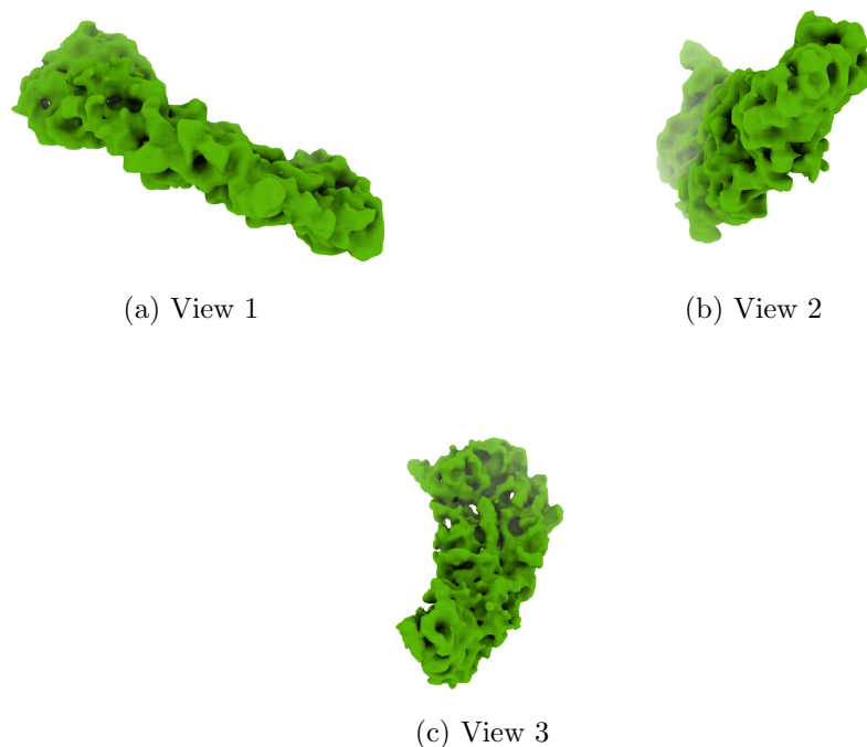
Figure 4: Isosurface at threshold=0.029800. Views generated by ChimeraX at a the following X, Y, Z angles: View 1 (0, -90, -90), View 2 (-90, 0, -90), View 3 (0, 0, 0).
