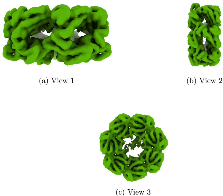
Figure 4: Isosurface at threshold=0.041000. Views generated by ChimeraX at a the following X, Y, Z angles: View 1 (0, -90, -90), View 2 (-90, 0, -90), View 3 (0, 0, 0).
