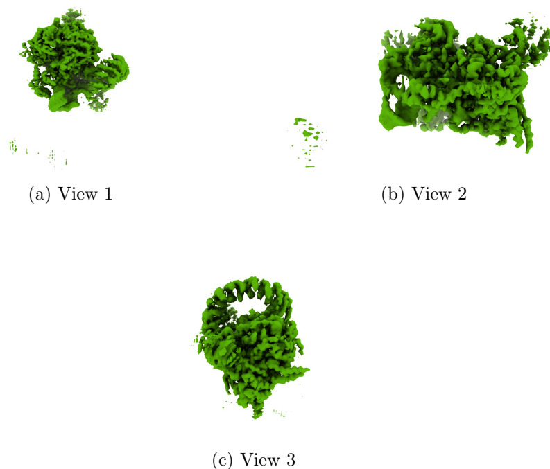
Figure 4: Isosurface at threshold=0.019900. Views generated by ChimeraX at a the following X, Y, Z angles: View 1 (0, -90, -90), View 2 (-90, 0, -90), View 3 (0, 0, 0).
