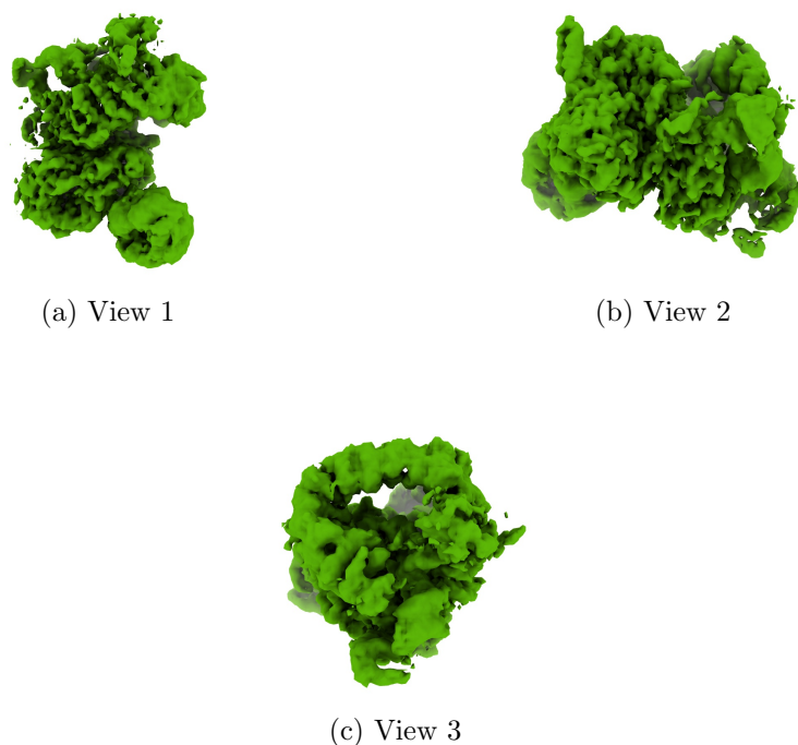
Figure 4: Isosurface at threshold=0.238000. Views generated by ChimeraX at a the following X, Y, Z angles: View 1 (0, -90, -90), View 2 (-90, 0, -90), View 3 (0, 0, 0).
