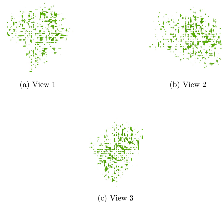
Figure 4: Isosurface at threshold=0.021800. Views generated by ChimeraX at a the following X, Y, Z angles: View 1 (0, -90, -90), View 2 (-90, 0, -90), View 3 (0, 0, 0).
