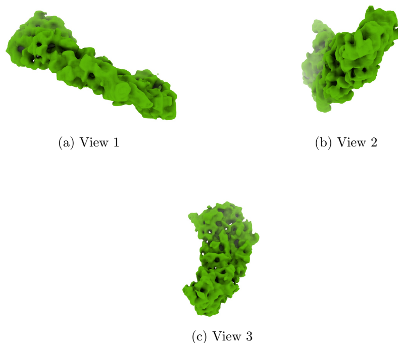
Figure 4: Isosurface at threshold=0.020400. Views generated by ChimeraX at a the following X, Y, Z angles: View 1 (0, -90, -90), View 2 (-90, 0, -90), View 3 (0, 0, 0).
