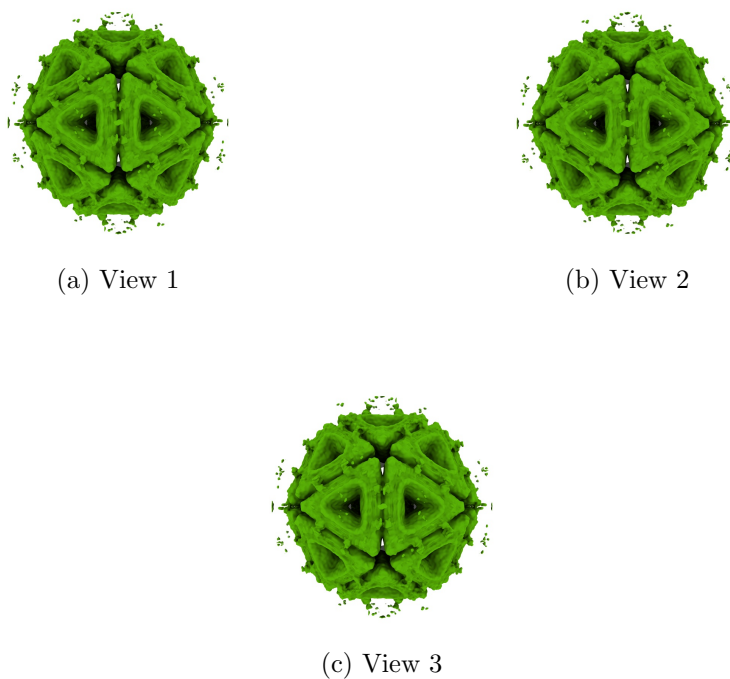
Figure 4: Isosurface at threshold=0.002740. Views generated by ChimeraX at a the following X, Y, Z angles: View 1 (0, -90, -90), View 2 (-90, 0, -90), View 3 (0, 0, 0).
