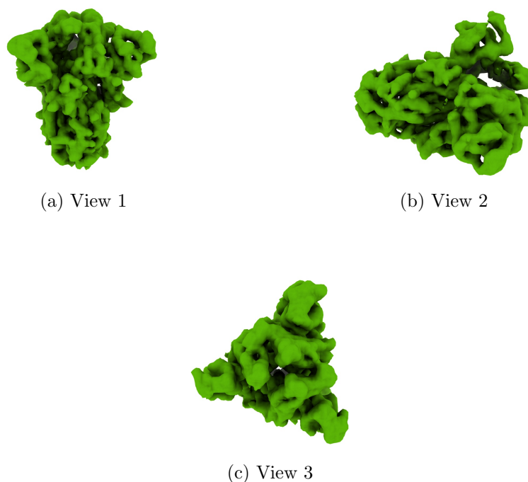
Figure 4: Isosurface at threshold=0.081000. Views generated by ChimeraX at a the following X, Y, Z angles: View 1 (0, -90, -90), View 2 (-90, 0, -90), View 3 (0, 0, 0).
