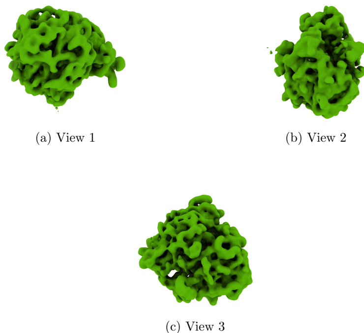
Figure 4: Isosurface at threshold=58.800000. Views generated by ChimeraX at a the following X, Y, Z angles: View 1 (0, -90, -90), View 2 (-90, 0, -90), View 3 (0, 0, 0).
