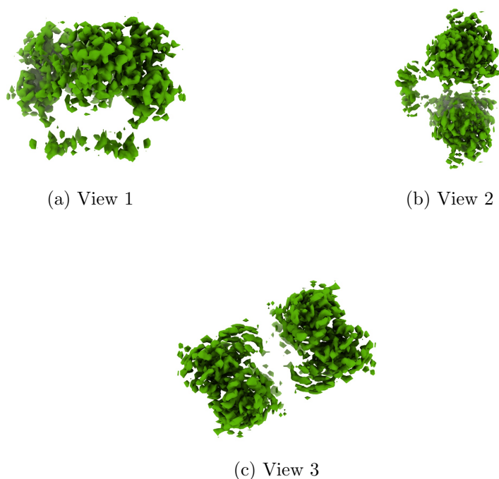
Figure 4: Isosurface at threshold=0.025300. Views generated by ChimeraX at a the following X, Y, Z angles: View 1 (0, -90, -90), View 2 (-90, 0, -90), View 3 (0, 0, 0).
