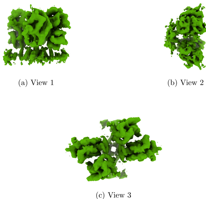
Figure 4: Isosurface at threshold=0.014300. Views generated by ChimeraX at a the following X, Y, Z angles: View 1 (0, -90, -90), View 2 (-90, 0, -90), View 3 (0, 0, 0).
