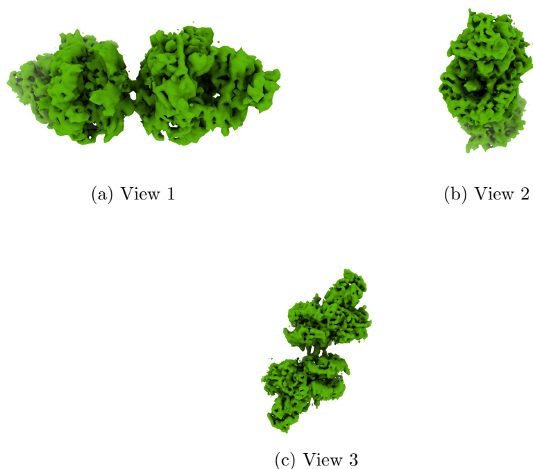
Figure 4: Isosurface at threshold=0.230000. Views generated by ChimeraX at a the following X, Y, Z angles: View 1 (0, -90, -90), View 2 (-90, 0, -90), View 3 (0, 0, 0).
