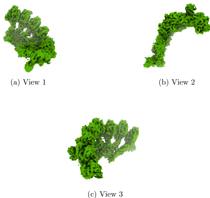
Figure 4: Isosurface at threshold=0.037900. Views generated by ChimeraX at a the following X, Y, Z angles: View 1 (0, -90, -90), View 2 (-90, 0, -90), View 3 (0, 0, 0).
