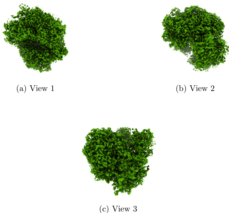
Figure 4: Isosurface at threshold=0.027000. Views generated by ChimeraX at a the following X, Y, Z angles: View 1 (0, -90, -90), View 2 (-90, 0, -90), View 3 (0, 0, 0).
