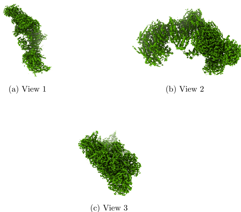
Figure 4: Isosurface at threshold=7.650000. Views generated by ChimeraX at a the following X, Y, Z angles: View 1 (0, -90, -90), View 2 (-90, 0, -90), View 3 (0, 0, 0).
