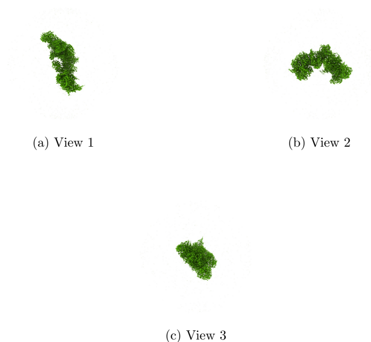
Figure 4: Isosurface at threshold=4.380000. Views generated by ChimeraX at a the following X, Y, Z angles: View 1 (0, -90, -90), View 2 (-90, 0, -90), View 3 (0, 0, 0).
