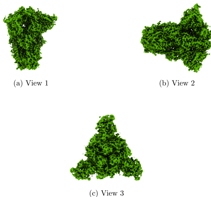
Figure 4: Isosurface at threshold=0.500000. Views generated by ChimeraX at a the following X, Y, Z angles: View 1 (0, -90, -90), View 2 (-90, 0, -90), View 3 (0, 0, 0).
