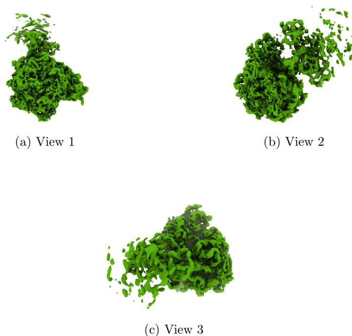
Figure 4: Isosurface at threshold=0.050900. Views generated by ChimeraX at a the following X, Y, Z angles: View 1 (0, -90, -90), View 2 (-90, 0, -90), View 3 (0, 0, 0).
