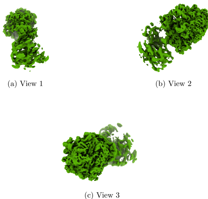
Figure 4: Isosurface at threshold=0.039600. Views generated by ChimeraX at a the following X, Y, Z angles: View 1 (0, -90, -90), View 2 (-90, 0, -90), View 3 (0, 0, 0).
