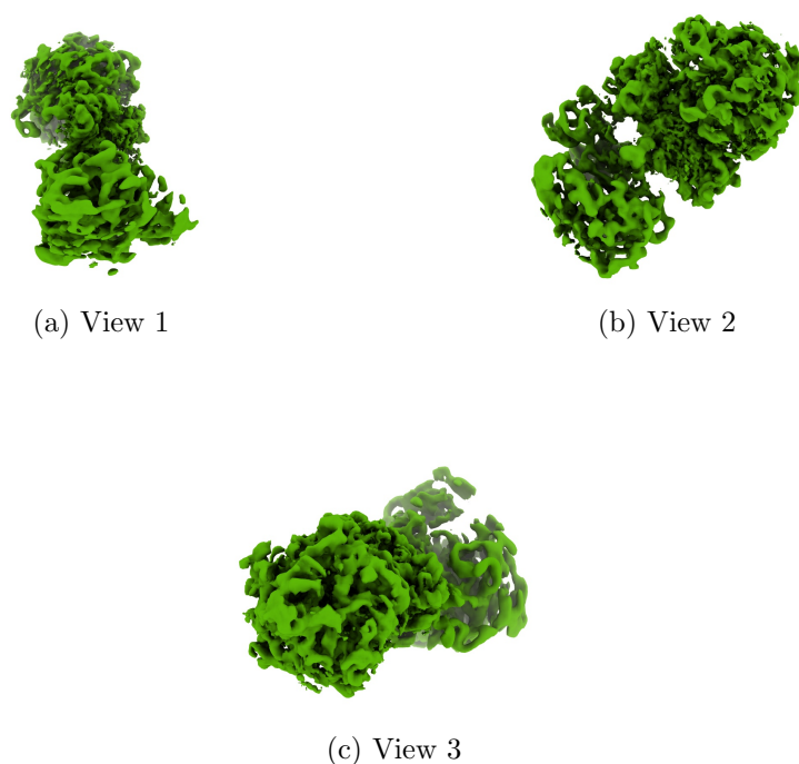
Figure 4: Isosurface at threshold=0.040100. Views generated by ChimeraX at a the following X, Y, Z angles: View 1 (0, -90, -90), View 2 (-90, 0, -90), View 3 (0, 0, 0).
