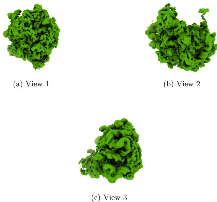
Figure 4: Isosurface at threshold=0.042500. Views generated by ChimeraX at a the following X, Y, Z angles: View 1 (0, -90, -90), View 2 (-90, 0, -90), View 3 (0, 0, 0).
