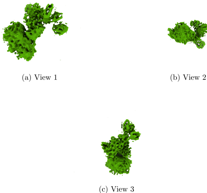
Figure 4: Isosurface at threshold=0.310000. Views generated by ChimeraX at a the following X, Y, Z angles: View 1 (0, -90, -90), View 2 (-90, 0, -90), View 3 (0, 0, 0).
