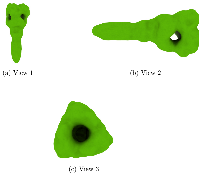
Figure 4: Isosurface at threshold=-95.000000. Views generated by ChimeraX at a the following X, Y, Z angles: View 1 (0, -90, -90), View 2 (-90, 0, -90), View 3 (0, 0, 0).
