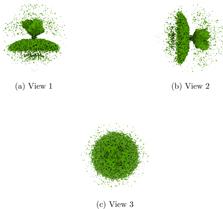
Figure 4: Isosurface at threshold=0.003130. Views generated by ChimeraX at a the following X, Y, Z angles: View 1 (0, -90, -90), View 2 (-90, 0, -90), View 3 (0, 0, 0).
