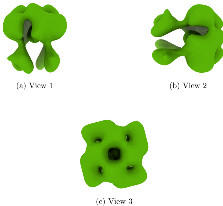
Figure 4: Isosurface at threshold=2.010000. Views generated by ChimeraX at a the following X, Y, Z angles: View 1 (0, -90, -90), View 2 (-90, 0, -90), View 3 (0, 0, 0).
