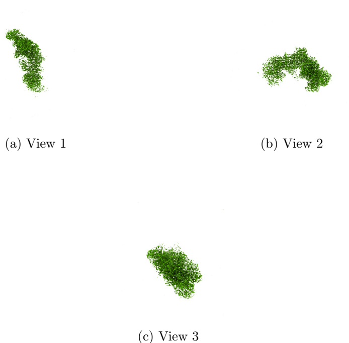
Figure 4: Isosurface at threshold=0.018000. Views generated by ChimeraX at a the following X, Y, Z angles: View 1 (0, -90, -90), View 2 (-90, 0, -90), View 3 (0, 0, 0).
