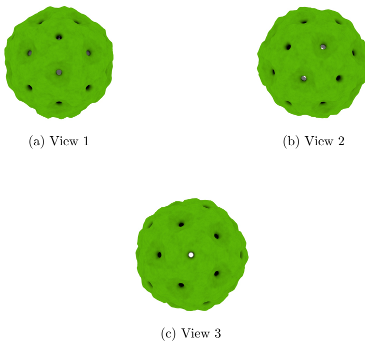
Figure 4: Isosurface at threshold=0.712000. Views generated by ChimeraX at a the following X, Y, Z angles: View 1 (0, -90, -90), View 2 (-90, 0, -90), View 3 (0, 0, 0).
