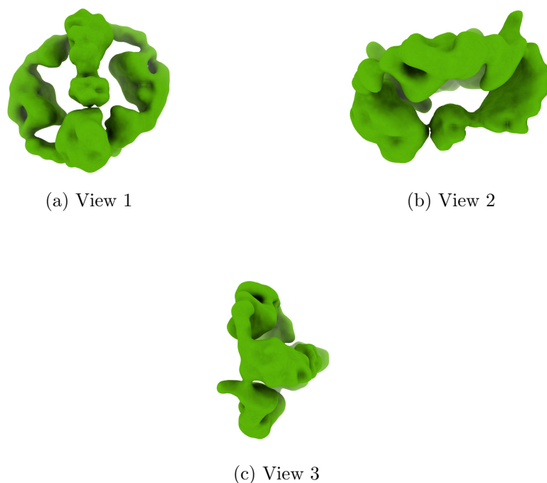
Figure 4: Isosurface at threshold=0.041400. Views generated by ChimeraX at a the following X, Y, Z angles: View 1 (0, -90, -90), View 2 (-90, 0, -90), View 3 (0, 0, 0).
