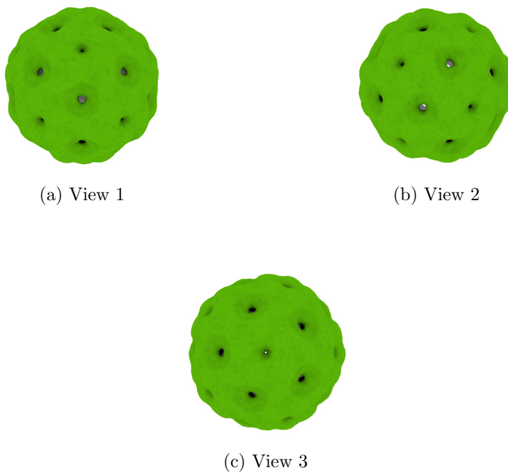
Figure 4: Isosurface at threshold=0.738000. Views generated by ChimeraX at a the following X, Y, Z angles: View 1 (0, -90, -90), View 2 (-90, 0, -90), View 3 (0, 0, 0).
