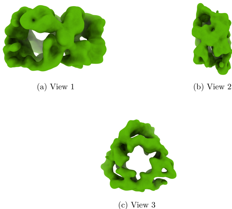
Figure 4: Isosurface at threshold=0.008610. Views generated by ChimeraX at a the following X, Y, Z angles: View 1 (0, -90, -90), View 2 (-90, 0, -90), View 3 (0, 0, 0).
