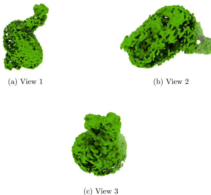
Figure 4: Isosurface at threshold=0.021500. Views generated by ChimeraX at the following X, Y, Z angles: View 1 (0, -90, -90), View 2 (-90, 0, -90), View 3 (0, 0, 0).
